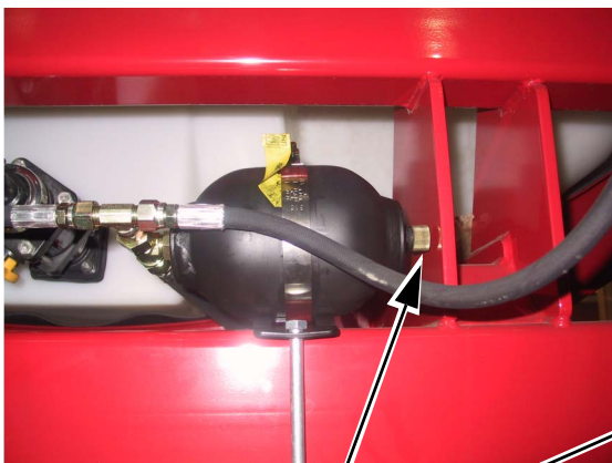
Boom rear rack accumulator Part# 600901512 version # 2
