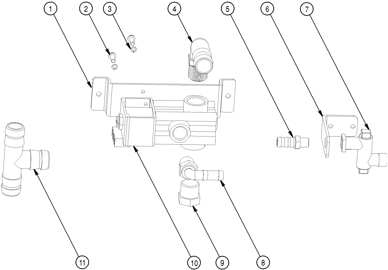
Fencerow Nozzle
