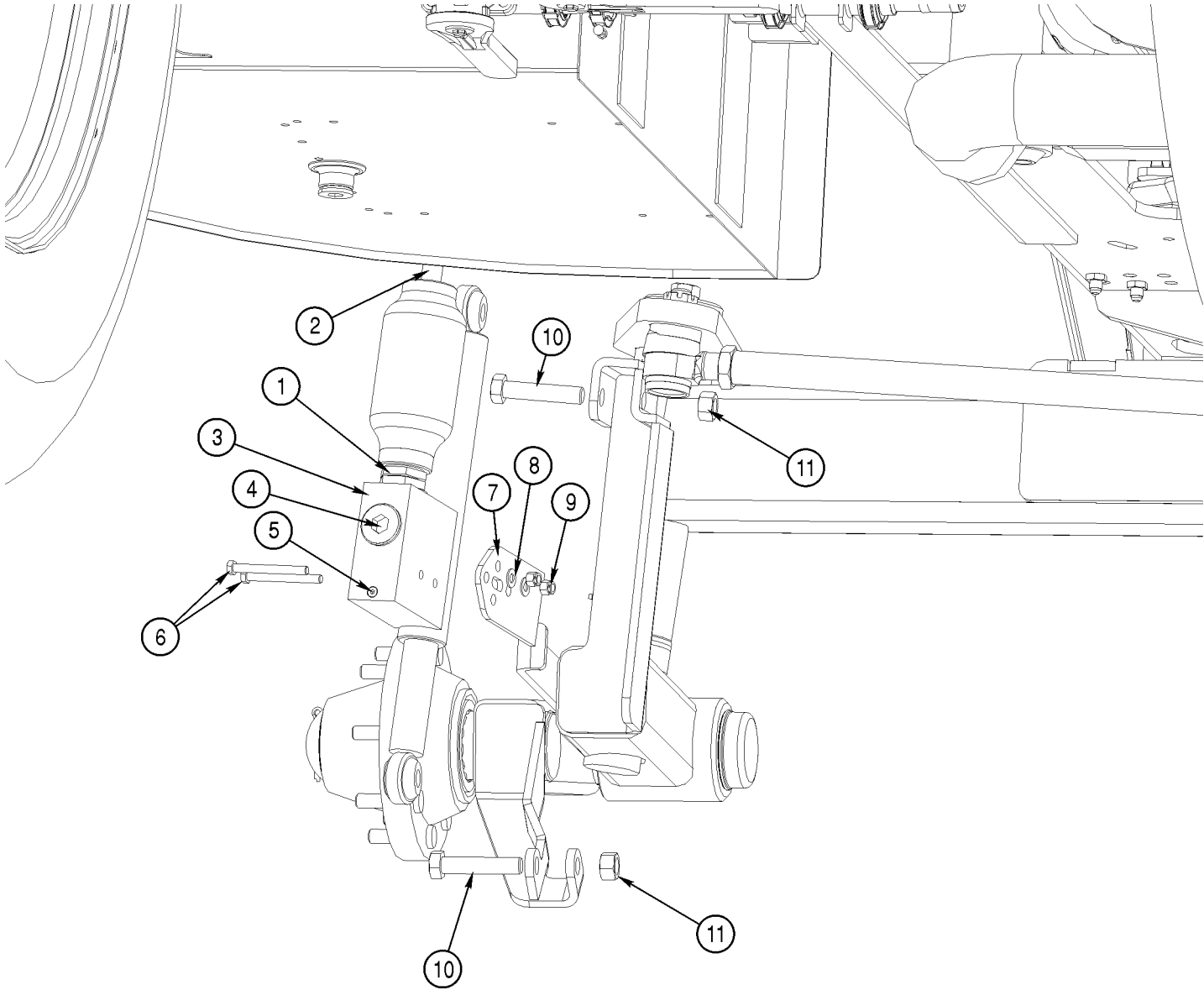
Front Strut AS710 & AS1010 (Standard Duty)
