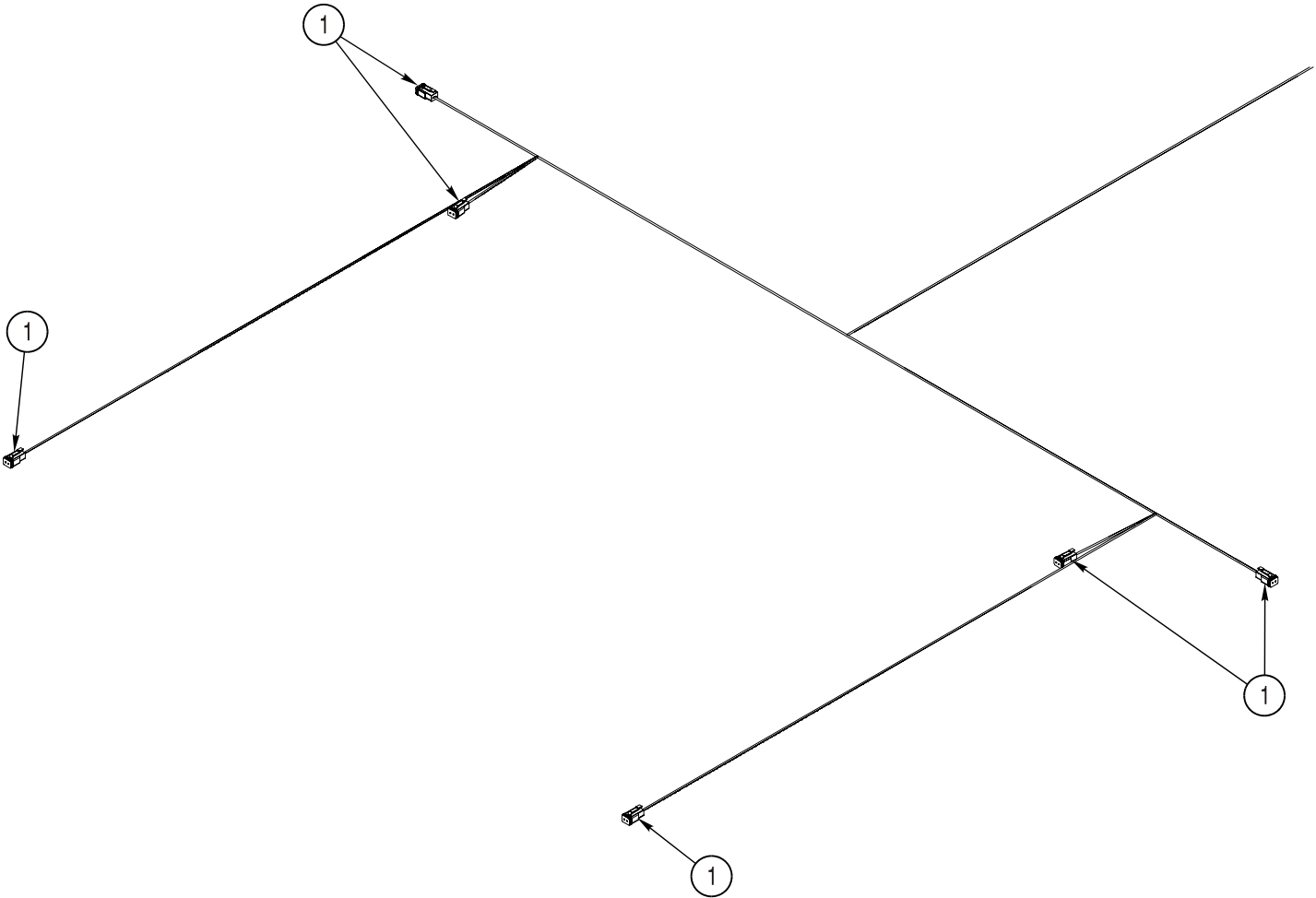
Auxiliary Cab Light Harness View 1
