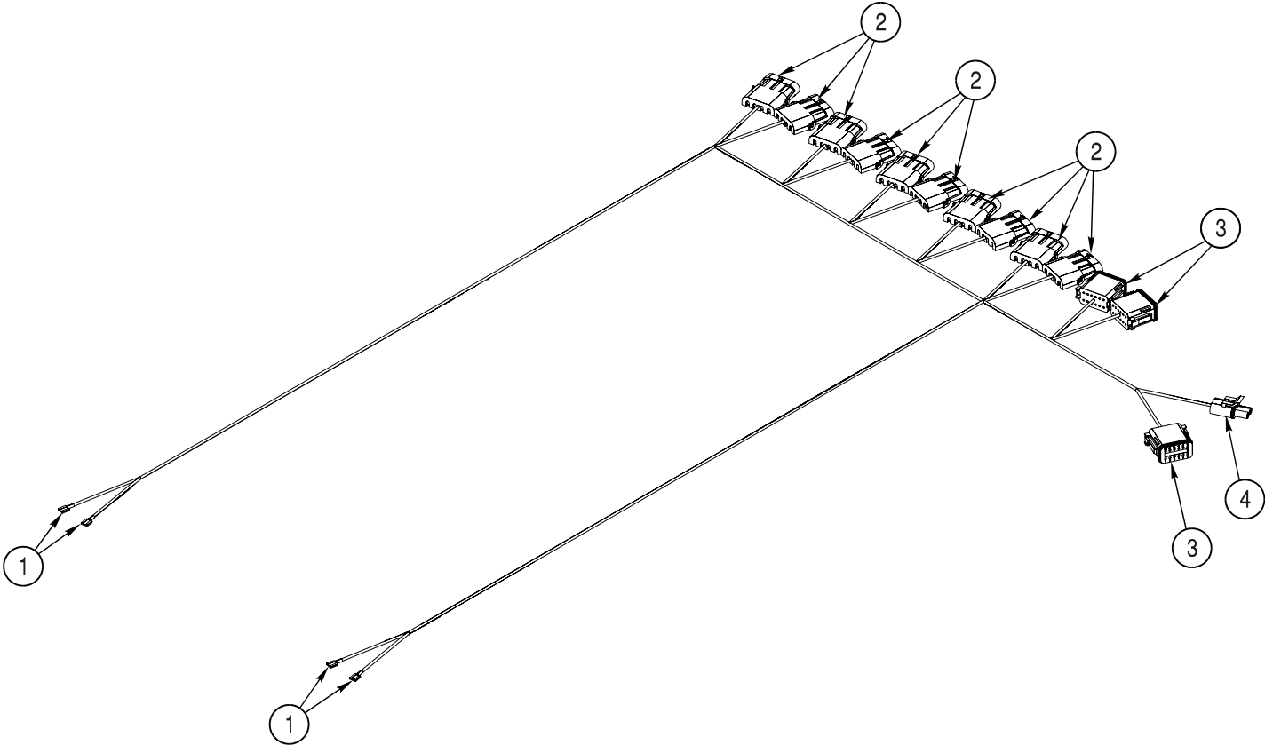
Boom Valve Harness
