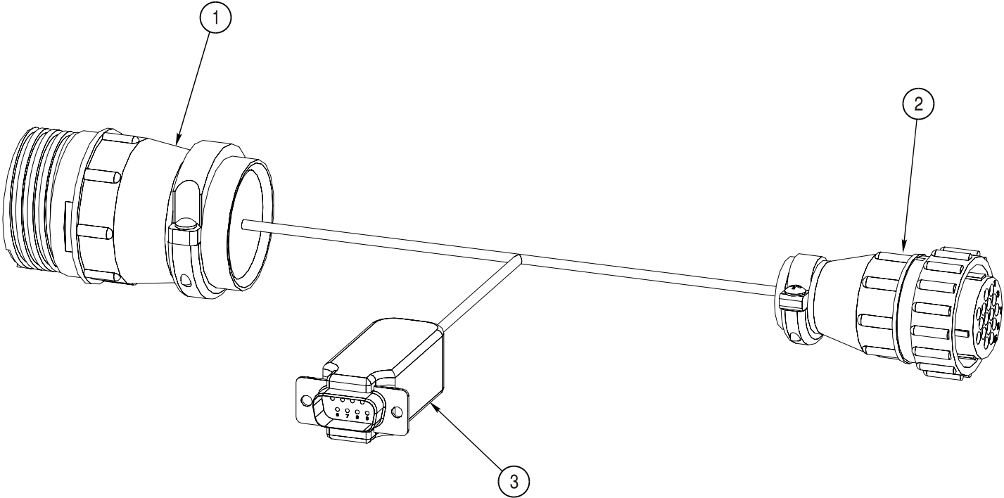
Raven 5000 to Viper E Pro Adapter Harness
