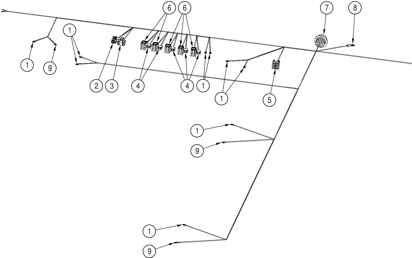
Cab Harness View 1 (Upper)
