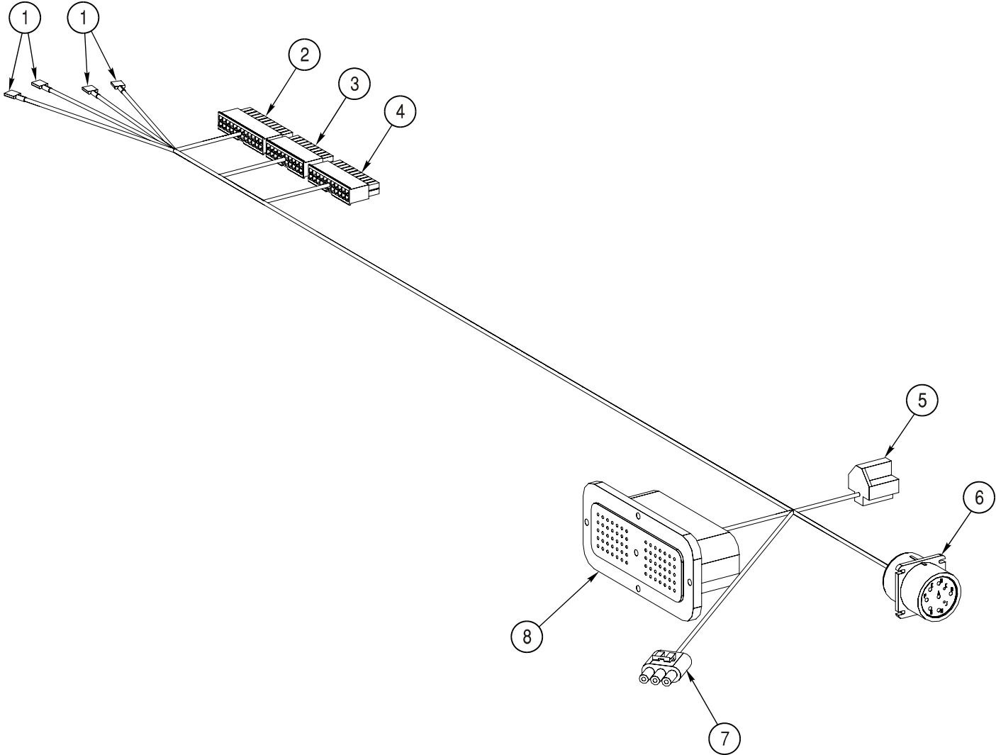
Funk Six Speed Console Harness
