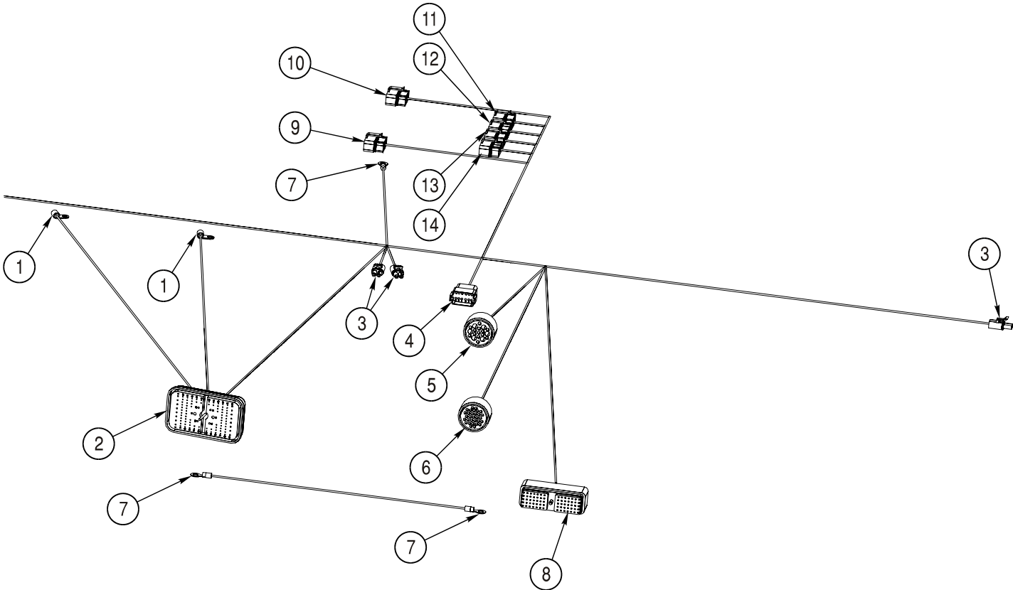
Cab Harness View 2 (Lower)
