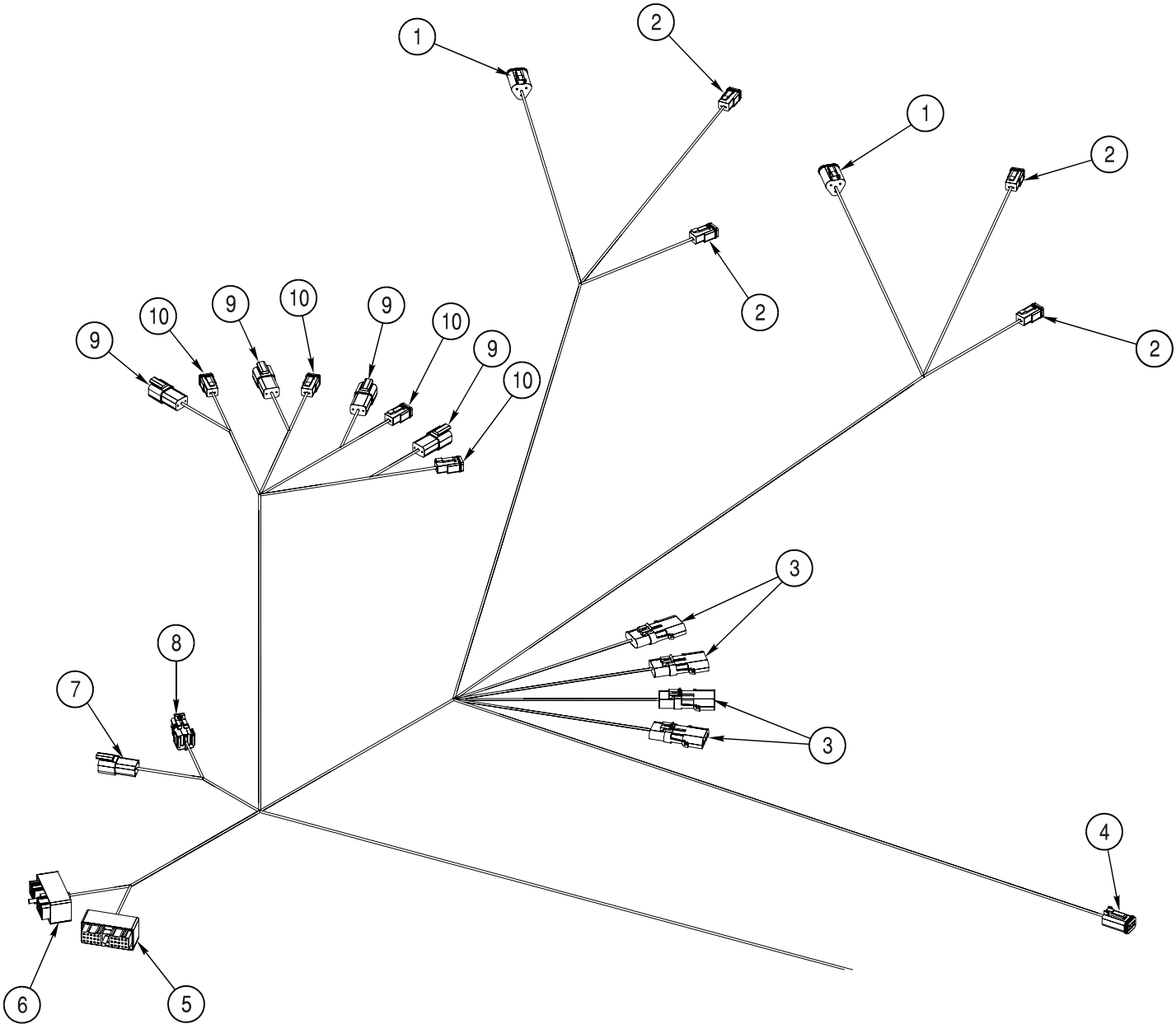
Autoboom Harness View 1
