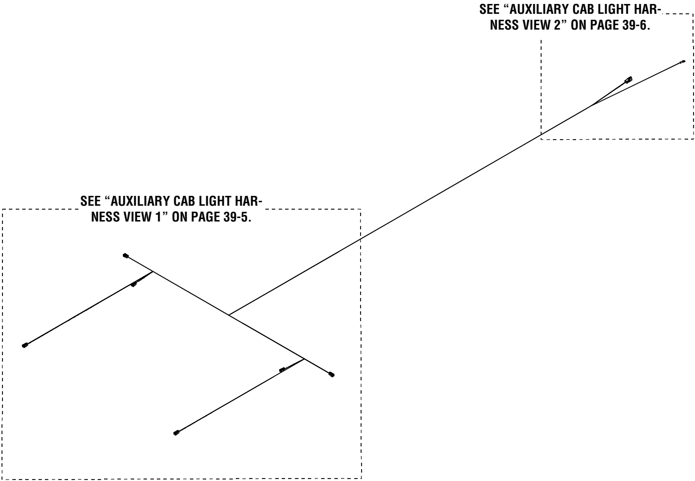
Auxiliary Cab Light Harness Overview
