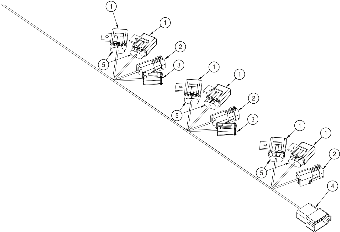
Raven Boom Control Harness View 1
