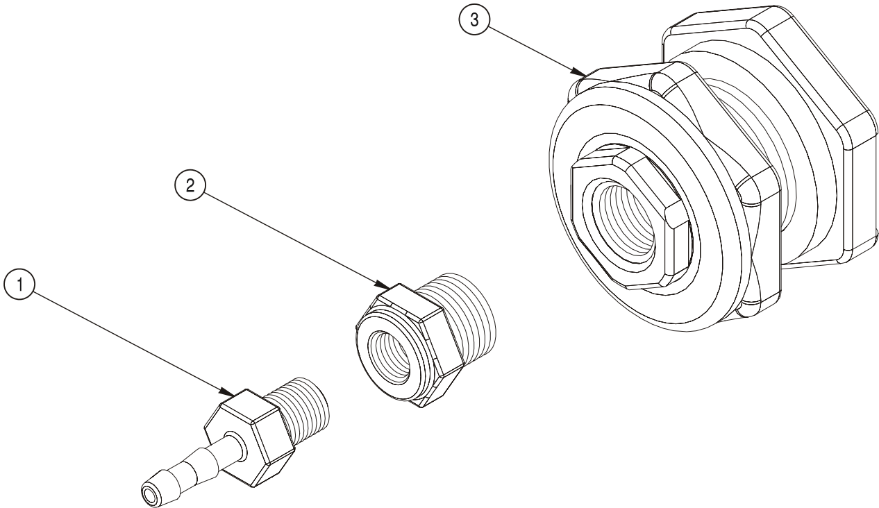
Foam Marker Rinse Tank Adapter (Smucker)
