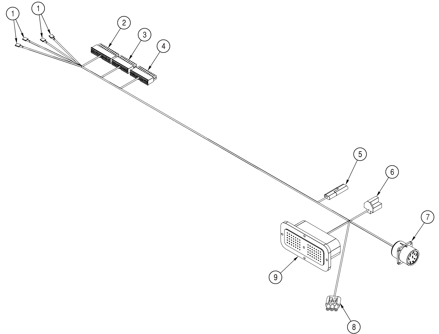
PowerShift 766 Harness
