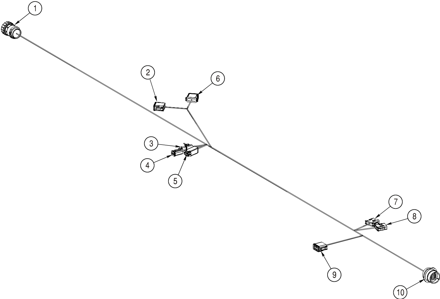
Raven Control Cab Harness
