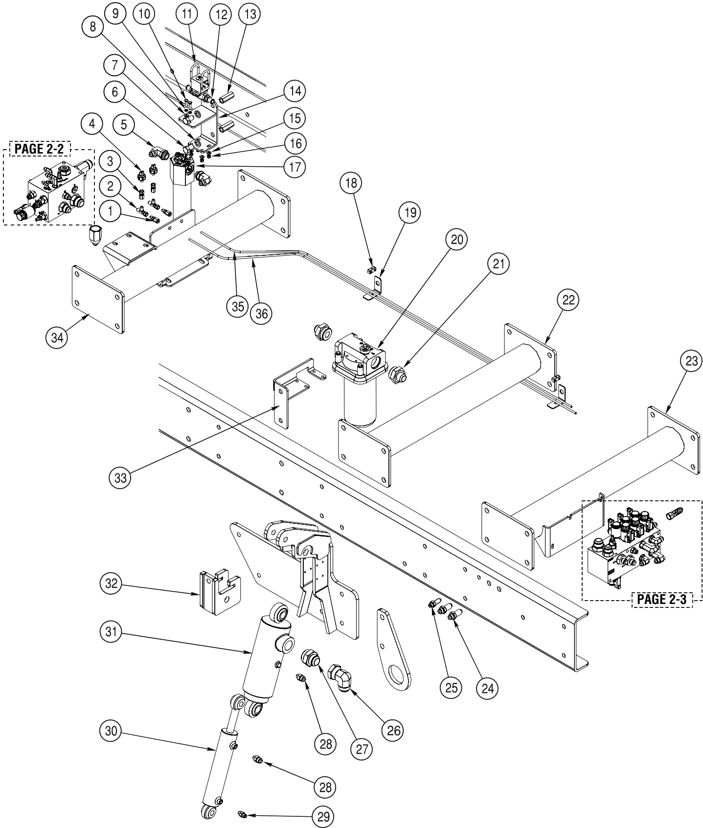
Frame Detail
