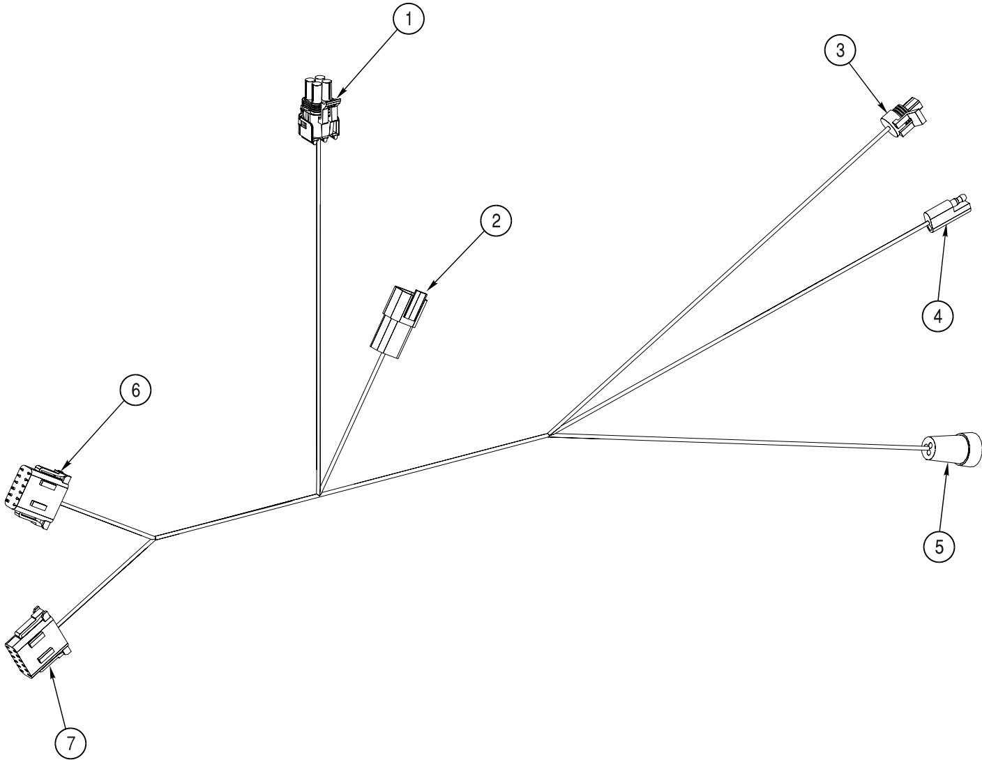
Can Control Node Harness
