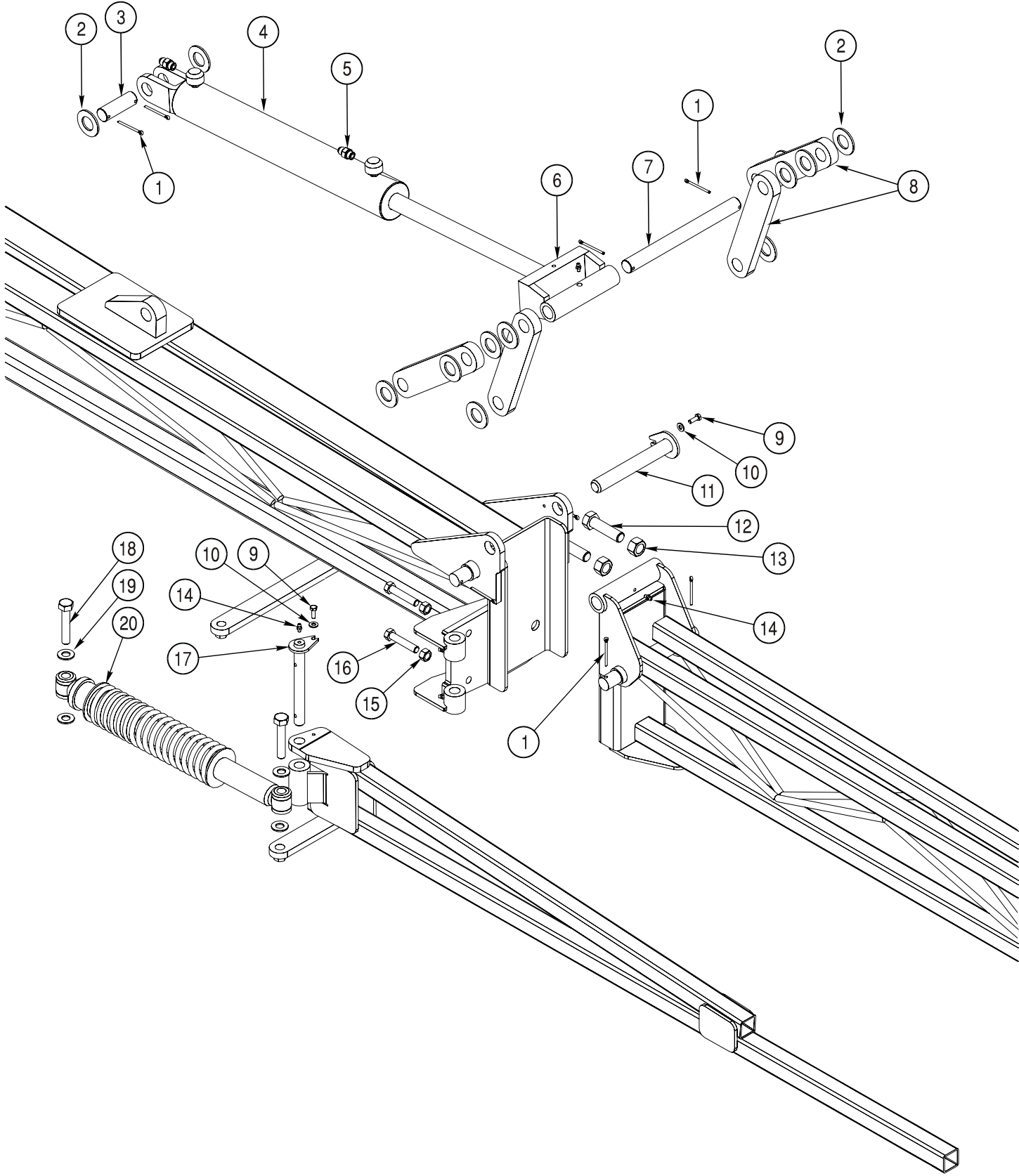
Boom Wing Inner Breakaway
